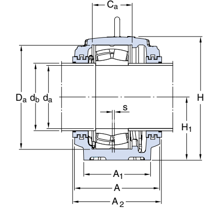
Labyrinth seals TS design
