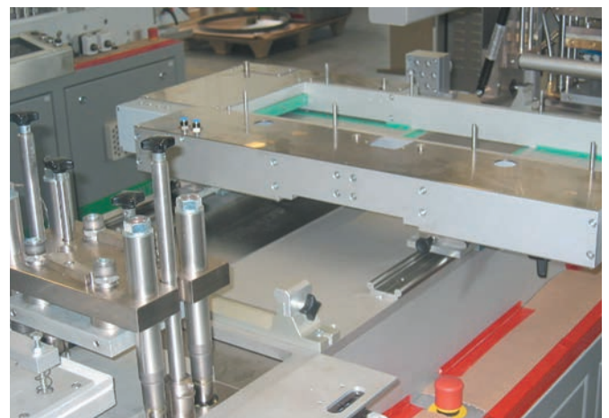
drylin® W is accredited to Cleanroom-standards and therefore used in this blister machine.
