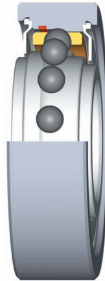
Dry Pump Bearing with Grease Reservoir
