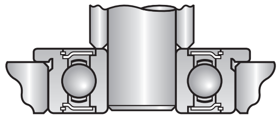
Fig. 1. Flanged bearings are recommended when housing designs cannot accommodate full bearing width or where the quality of housing bore is a concern.
