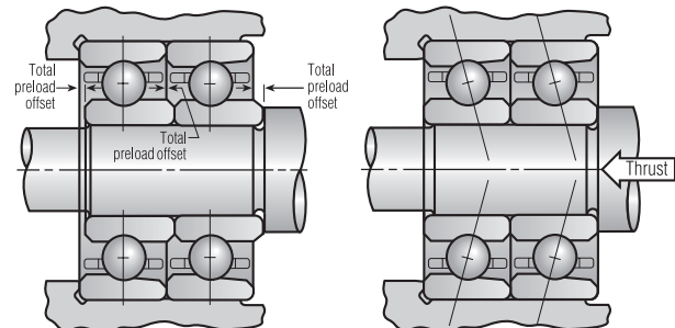
Fig. 11. DT mounting.
